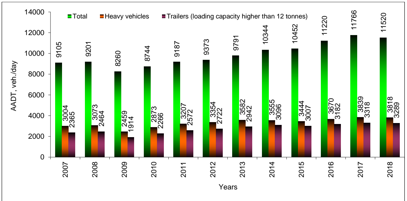
Change of annual average daily traffic (AADT) on the transport corridor Via Baltica since 2007
