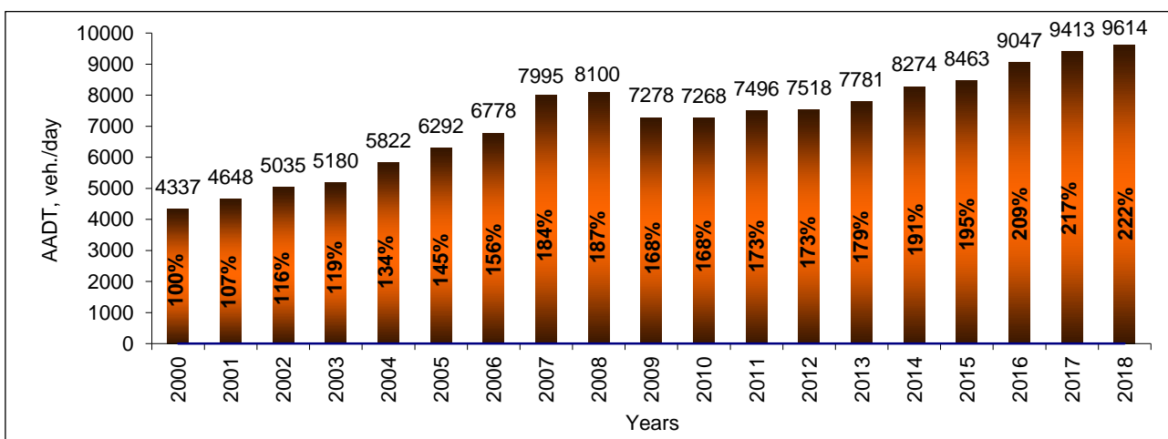
Change of annual average daily traffic (AADT) on the main roads, compared to the year 2000
