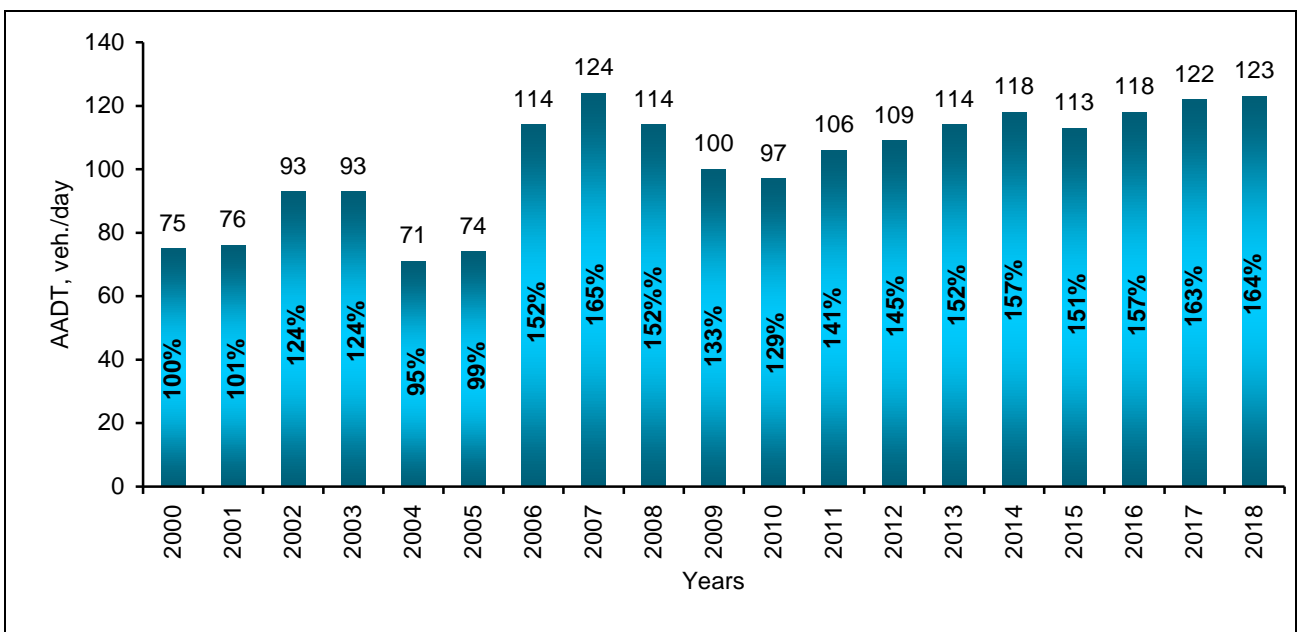
Change of trailer (loading capacity higher than 12 tonnes) average daily traffic (AADT) on the national roads, compared to the year 2000
