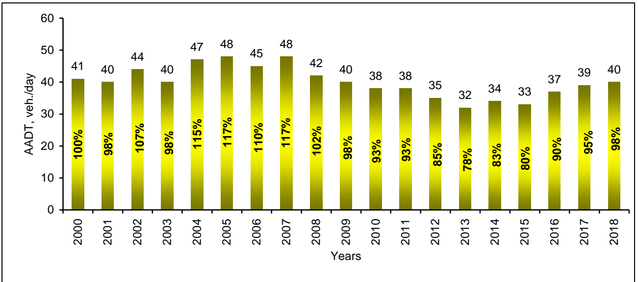
Change of heavy vehicles' annual average daily traffic (AADT) on the regional roads, compared to the year 2000
