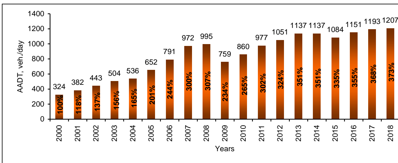
Change of trailer (loading capacity higher than 12 tonnes) annual average daily traffic (AADT) on the main roads, compared to the year 2000
