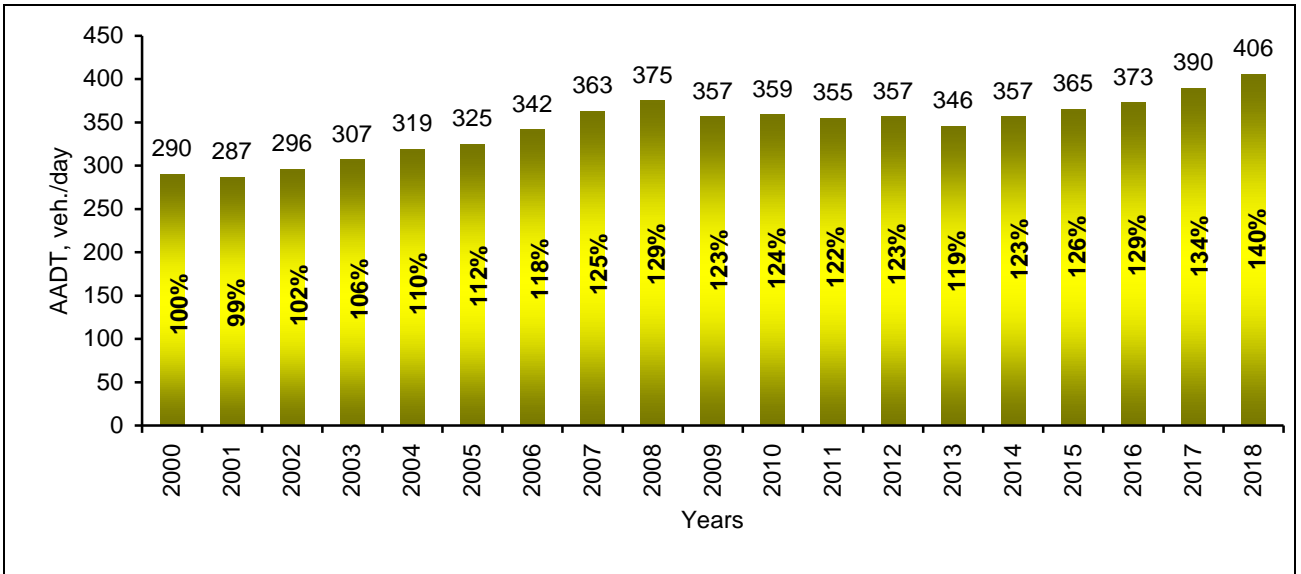
Change of annual average daily traffic (AADT) on the regional roads, compared to the year 2000
