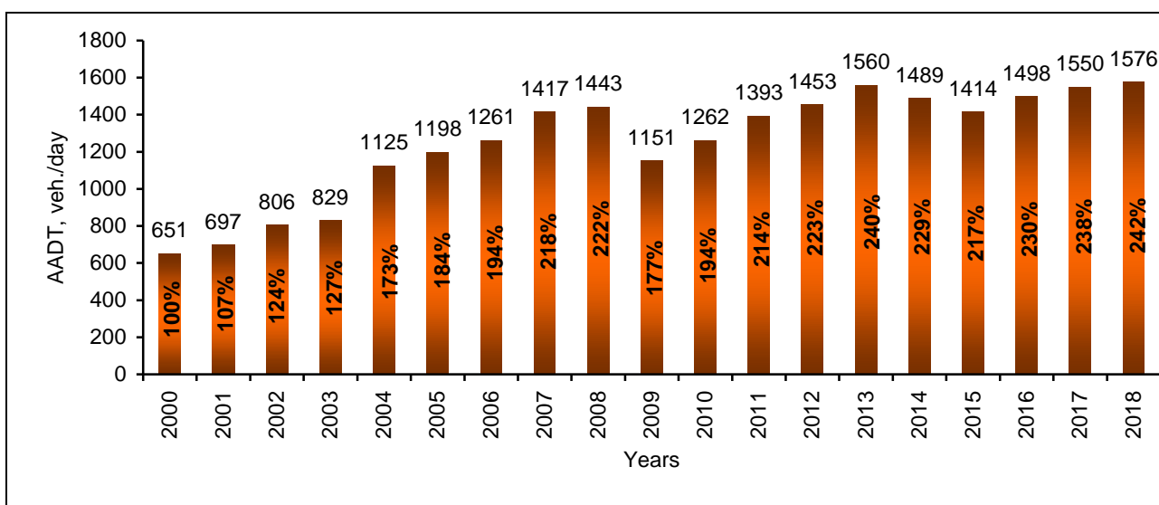
Change of heavy vehicles' annual average daily traffic (AADT) on the main roads, compared to the year 2000
