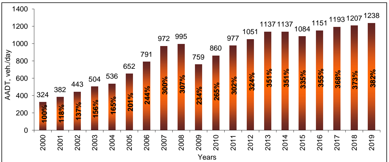
Change of trailer (loading capacity higher than 12 tonnes) annual average daily traffic (AADT) on the main roads, compared to the year 2000
