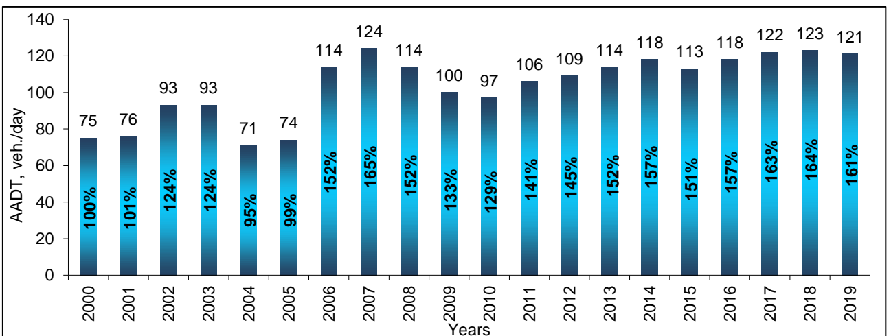
Change of trailer (loading capacity higher than 12 tonnes) average daily traffic (AADT) on the national roads, compared to the year 2000
