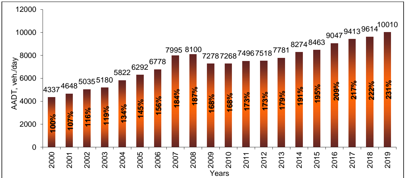
Change of annual average daily traffic (AADT) on the main roads, compared to the year 2000
