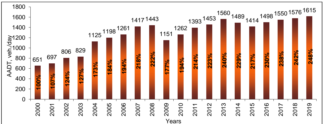
Change of heavy vehicles' annual average daily traffic (AADT) on the main roads, compared to the year 2000
